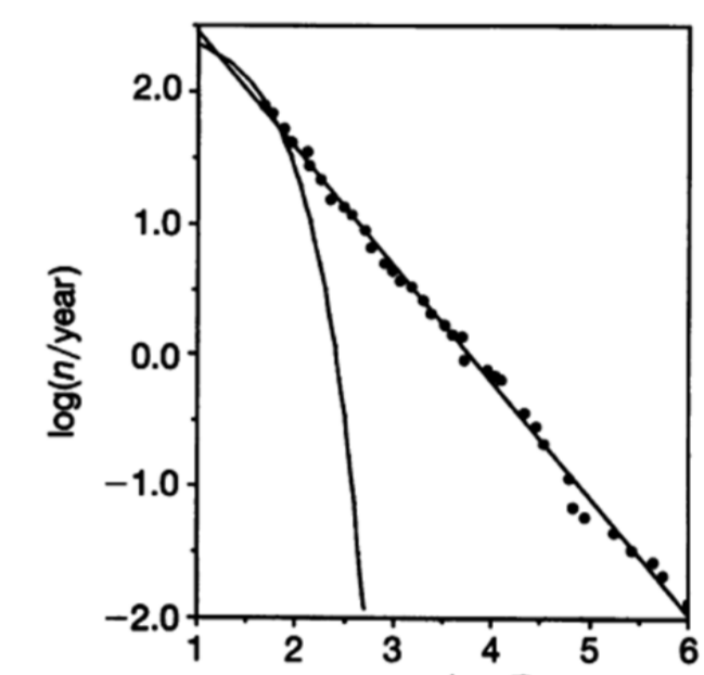
Distribution of earthquakes in the New Madrid zone in the southeastern United States during the period 1974-1983, collected by Johnson and Nava. P. Bak and M. Paczuski, Proc. Natl. Acad. Sci. USA, Vol 92, 1995.
